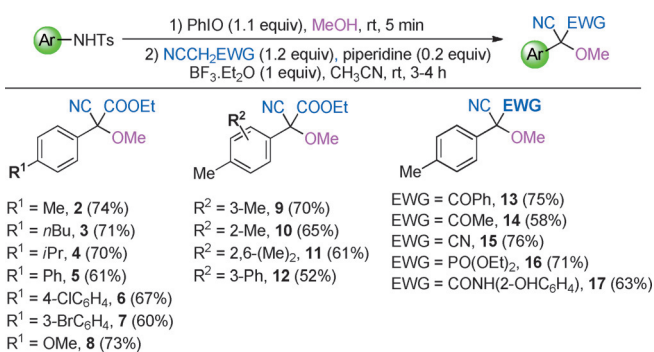
Scheme 3. Investigation of the scope of anilines and nitriles.
